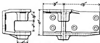
Figs. 3736-3738. Safety Bar Bracket.
